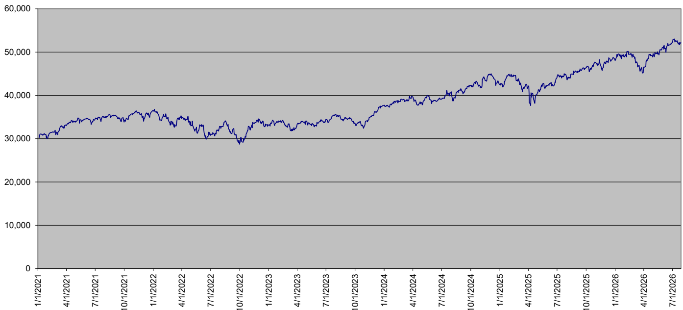
INDU Index Daily Closing Levels January 1, 2021 to July 27, 2026
